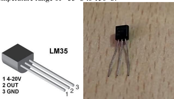
Fig.4 Temperature Sensor
