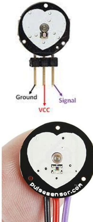
Fig.3 Heartbeat Sensor
