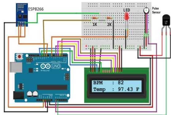
Fig.8 Components connections
