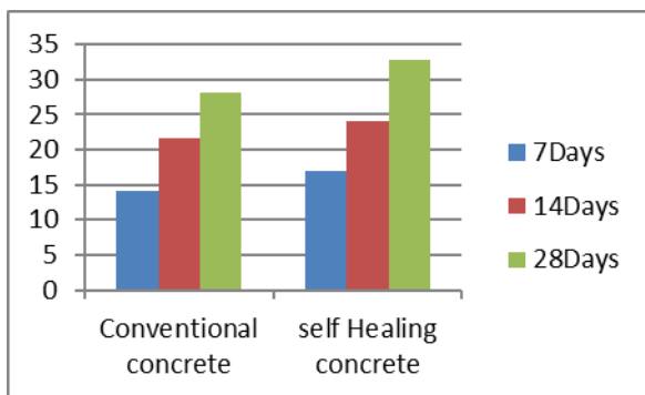
Fig. 3 Effect of bacillus Subtilis bacteria on Compressive strength
