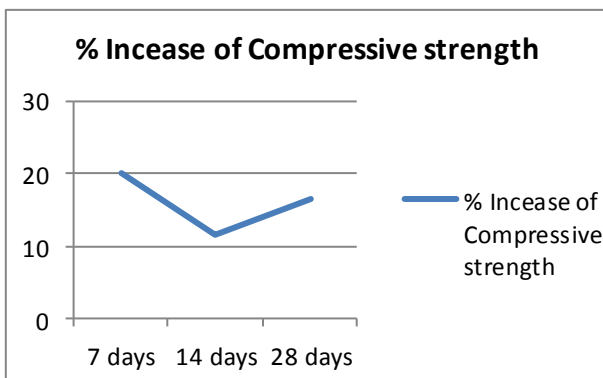
Fig.4 % Increase in Compressive strength of self healing concrete with ages
