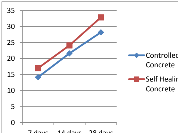
Fig. 2 Comparison of Compressive Strength of Controlled and Self healing concrete
