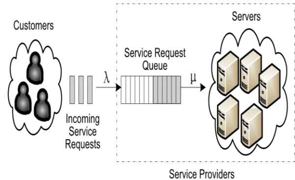
Fig. 1. Cloud Computing Service Queuing Model
