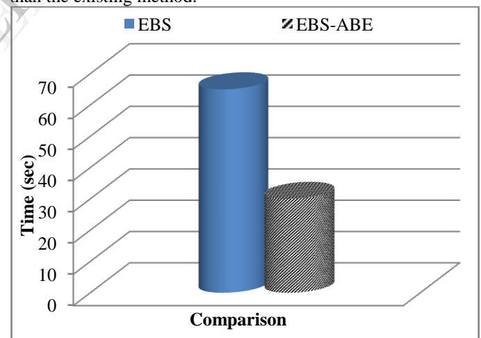
Fig.5. Execution time for EBS-ABE (proposed) and EBS (existing)
