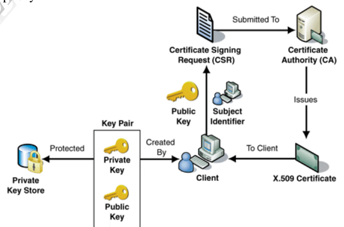
Fig.1 Public key infrastructure for secure communication
