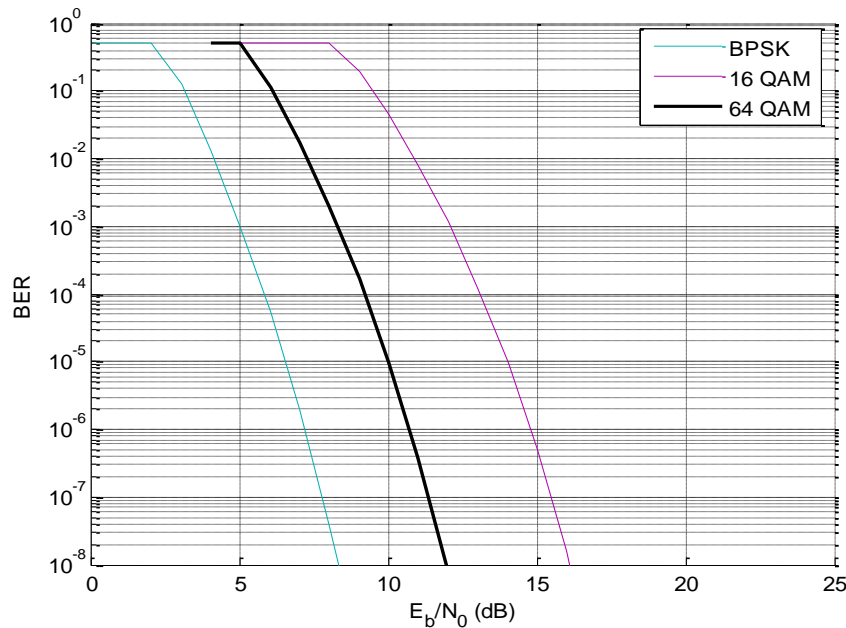
Figure 4: PLOT OF BER V/S Eb/No. FOR DIFFERENT MODULATION TECHNIQUE
