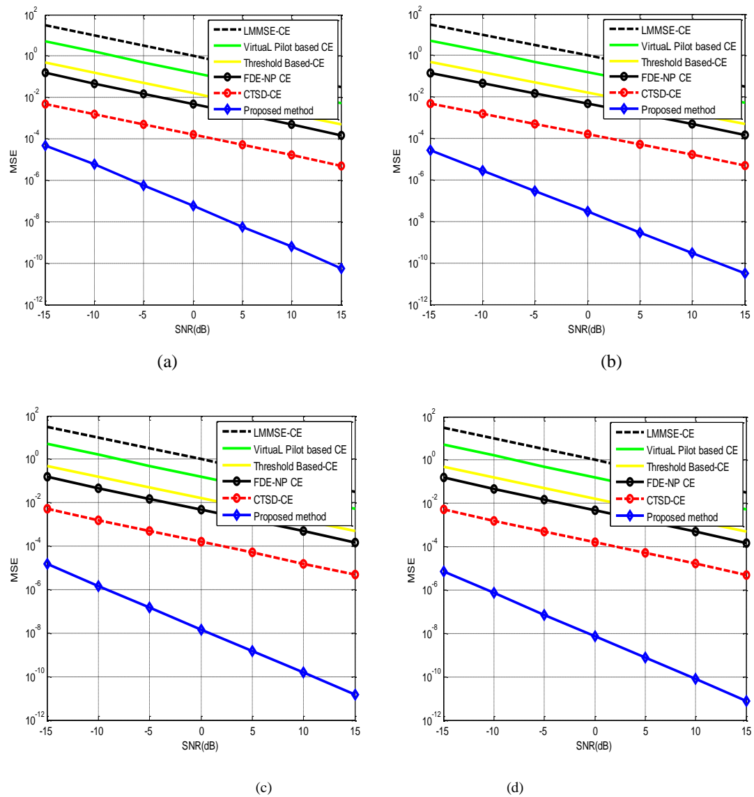
Figure 3: MSE V/S SNR plot for 64-QAM modulation (a) N=64, L=8 , (b) N=128, L=8 , (c) N=256, L=8 & (d) N=512, L=8
