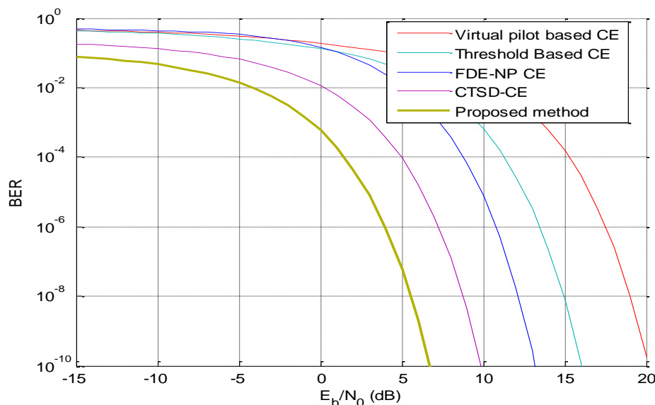
Figure 5: BER Performance of the conventional and proposed Method for 64 QAM Modulation scheme
