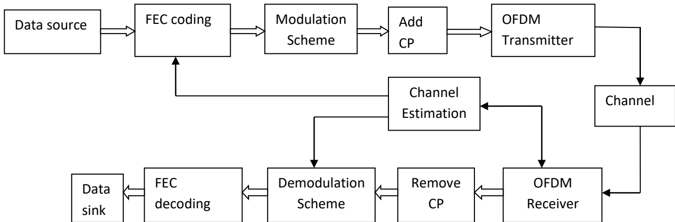
Figure 1: BLOCK DIAGRAM OF PROPOSED METHOD
