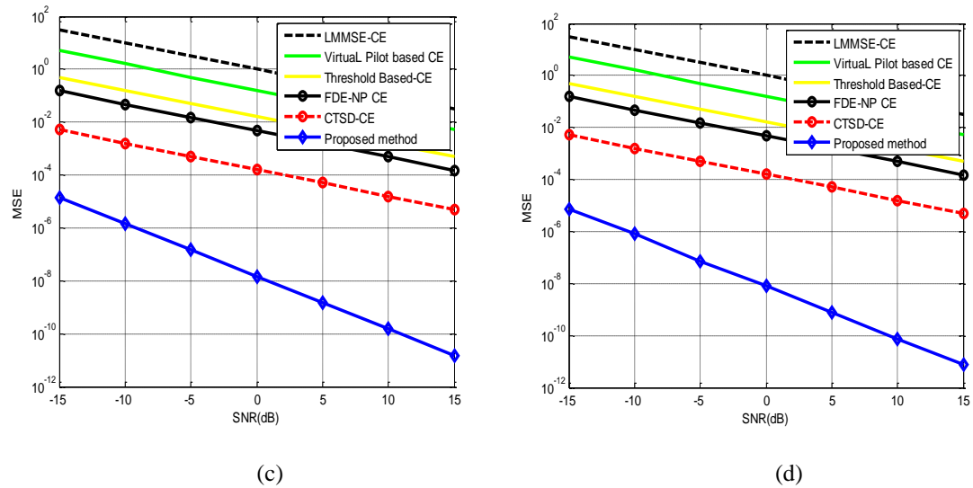
Figure 2: MSE V/S SNR plot for 64-QAM modulation (a) N=64, L=4 , (b) N=128, L=4 , (c) N=256, L=4 & (d) N=512, L=4
