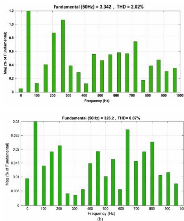
Figure 12. (a) Source current THD with NARMA-L2 controller. (b) Load voltage THD with NARMA L2 controller
