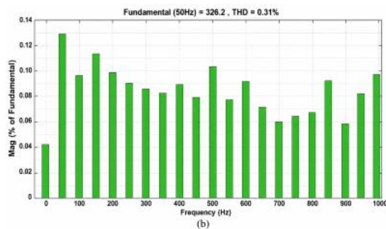
Figure 11. (a) Source current THD PI controller with adaptive lizard algorithm (b) Load voltage THD PI controller with adaptive lizard algorithm
