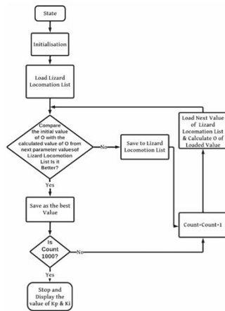
Figure 5. Flow chart to find the parameters using adaptive lizard algorithm (ALA)
