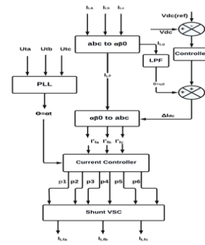
Figure 3. Control structure of shunt compensator Controllers
