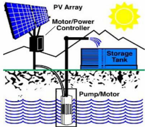
Fig. 5 A typical solar-powered stock watering system
