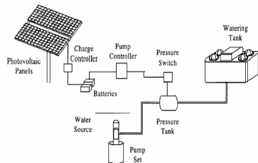
Fig. 3 Battery-coupled solar water pumping system determining the optimum system for a particular application.
