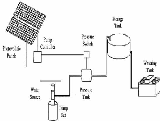
Fig. 4 Direct coupled solar pumping system
