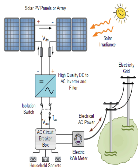
Fig. 4 : Grid system
