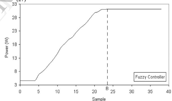
Figure 7. Sample versus power of PV array, using fuzzy controller method. At point B, the fuzzy controller’s method reaches MPP after iteration (24).
