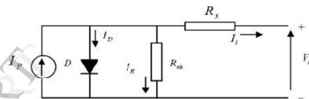
Figure 3: Equivalent circuit of a solar cell
