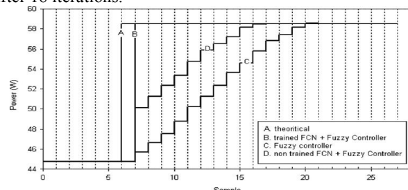
Figure 15. Sample versus power of PV-array. (A) Theoretical, (B) proposed method (off-line trained FCN), (C) fuzzy controller, and (D) proposed method (only on-line trained FCN).
