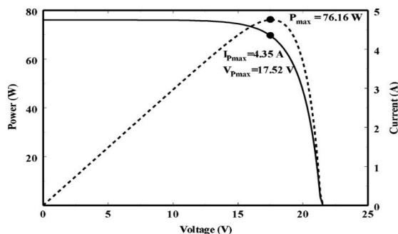
Figure 1: PV array (I-V) and P-V characteristics
