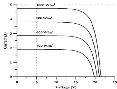
Figure 2: PV array (I-V) characteristics at various insolation levels
