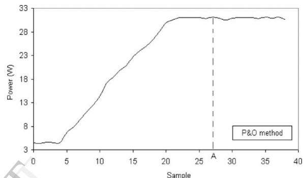
Figure 6. Sample versus power of PV array using P&O method. At point A, the P&O method reaches the MPP for first time after iteration (27)
