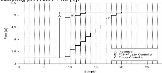
Figure 13. Sample versus power of PV-array. (A) Theoretical, (B) proposed method, and (C) fuzzy controller
