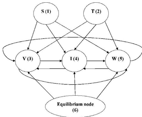
Figure. 9 FCN Designed for the photovoltaic project
