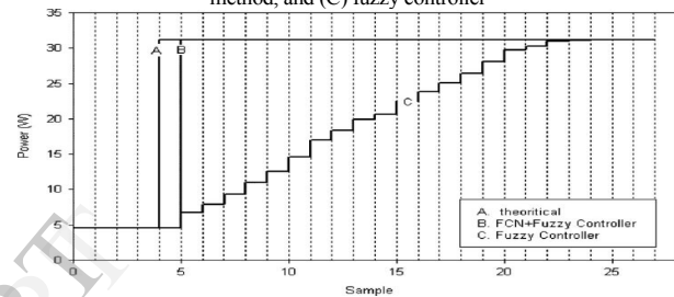
Figure 14. Sample versus power of PV-array. (A) Theoretical, (B) proposed method, and (C) fuzzy controller
