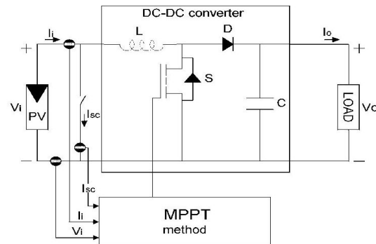
Figure. 5. Step-up boost converter for MPPT.
