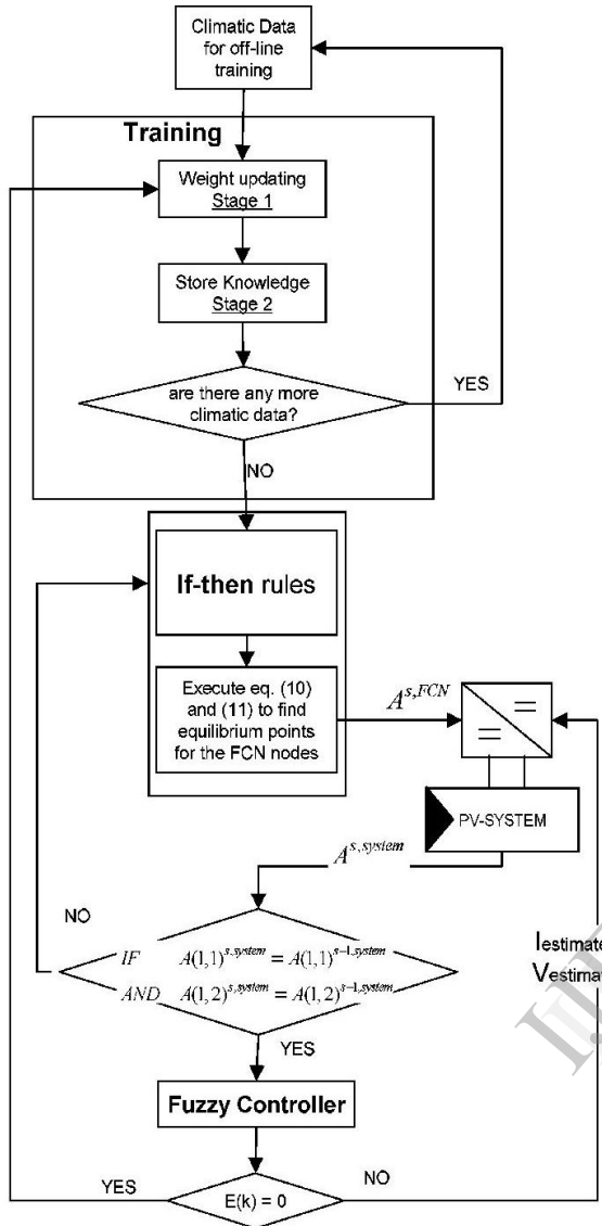
Figure10: simplified flowchart of the proposed method
