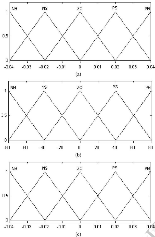
Figure 4. Membership function for (a) input E(k); (b) input CE(k); (c) output dD.
