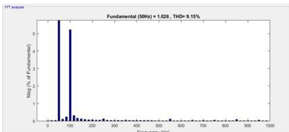
Fig. 6V_l Fuzzy with 0.1s start time
