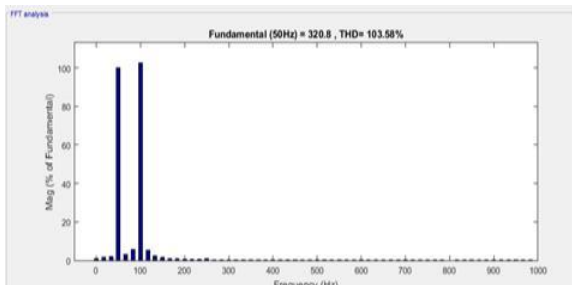
Fig. 4 i_l Fuzzy with 0.1s start time
