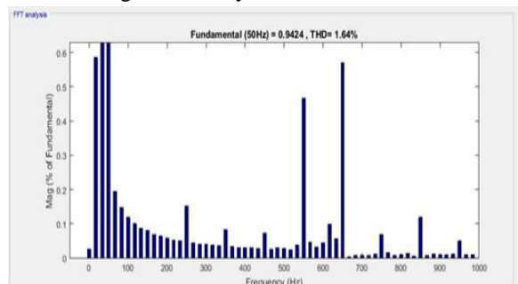
Fig. 10V_l Fuzzy with 0.5s start time
