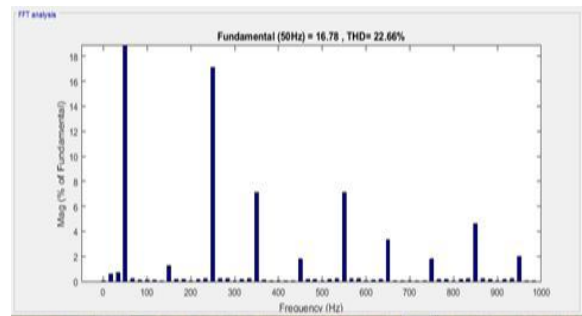
Fig. 8i_l Fuzzy with 0.5s start time
