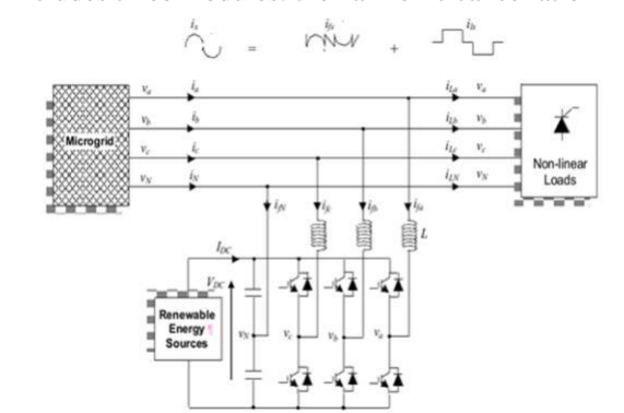
Fig-2 APC Topology
