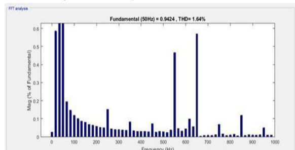
Fig. 11V_s Fuzzy with 0.5s start time
