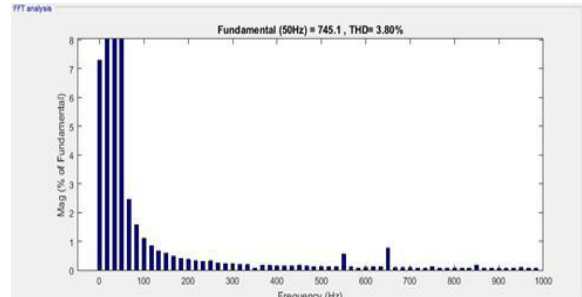
Fig. 9i_s Fuzzy with 0.5s start time
