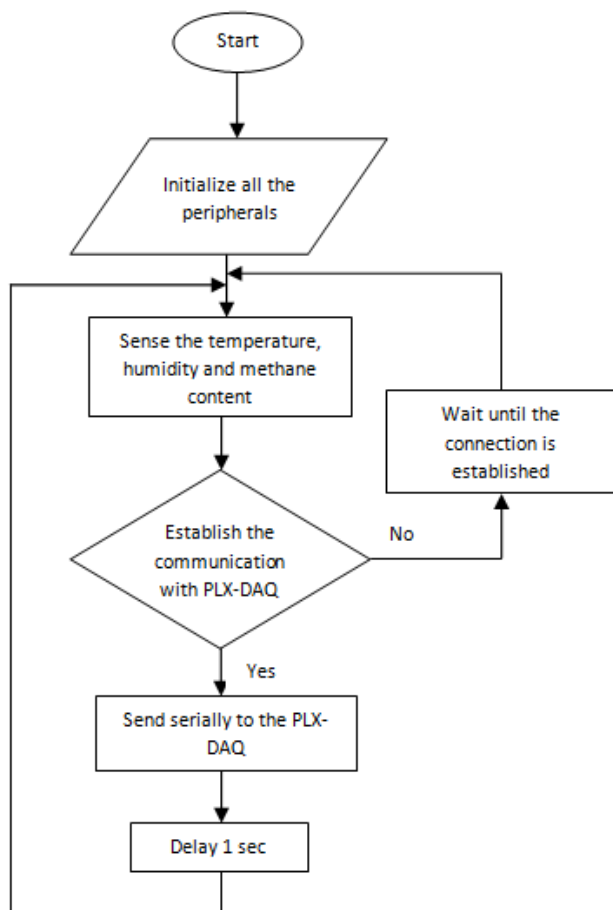
Fig. 2. Flow chart of the data acquisition process
