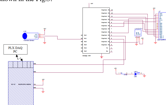
Fig.3. Circuit Diagram of Data Acquisition module
