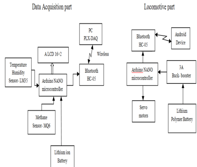
Fig. 1. Block Diagram of the data acquisition part and the locomotive part
