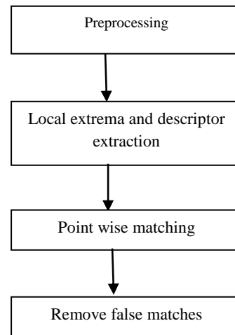
Fig. 6: Flow chart of sift algo
