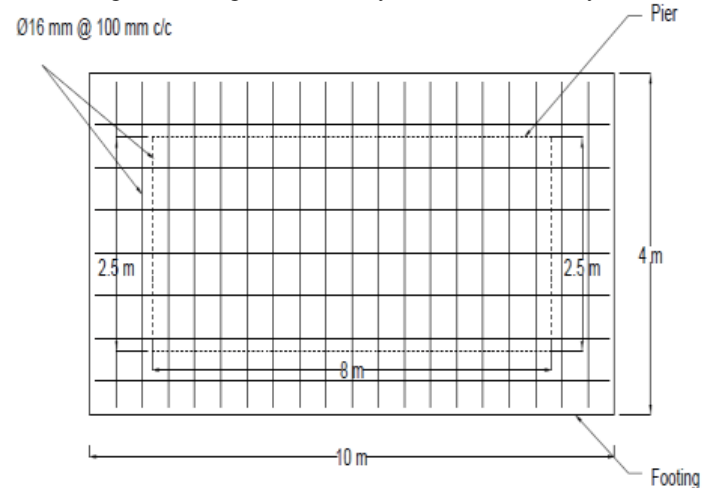
Fig. 14: Footing for Pier
