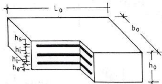
Fig. 11: Elastomeric rubber pad bearing
