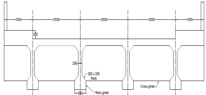
Fig. 1: Cross section of the bridge deck
