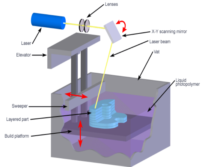
Fig. 5. Stereolithography
