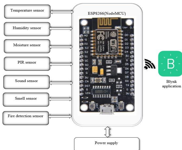
Fig 1: Block diagram of smart warehouse management system
