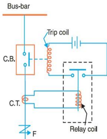
Fig. 5. Typical Relay Circuit Diagram
