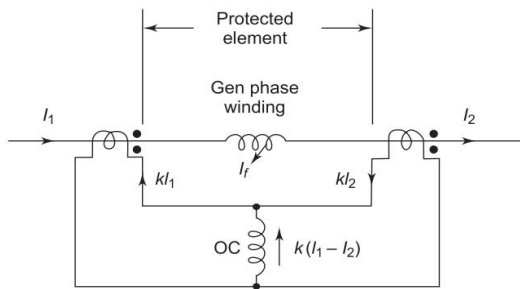
Fig. 8. Differential protection scheme
