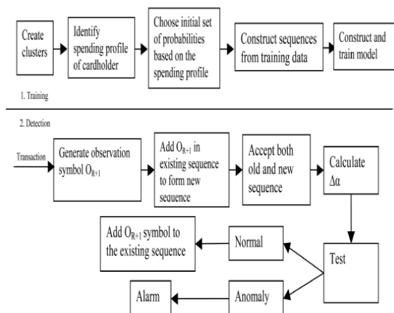
“Figure 1. Architecture of Hidden Markov model”
