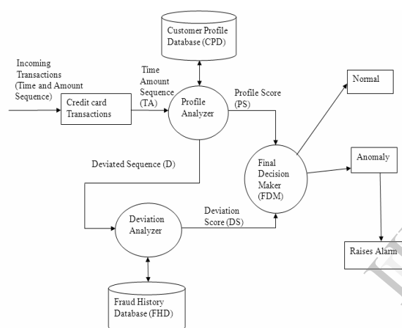
“Figure 2. Architecture of BLAST-SSAHA fraud detection system”
