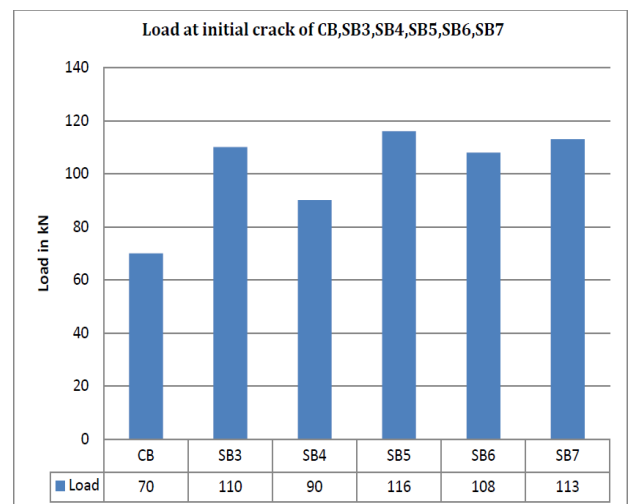
Figure : Result obtained by author showing the load at initial crack of control beam and strengthened beam
