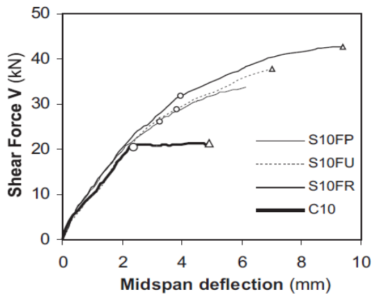
Figure1 Load deflection curve obtained by author for control beam with web reinforcement and shear strengthened beam
