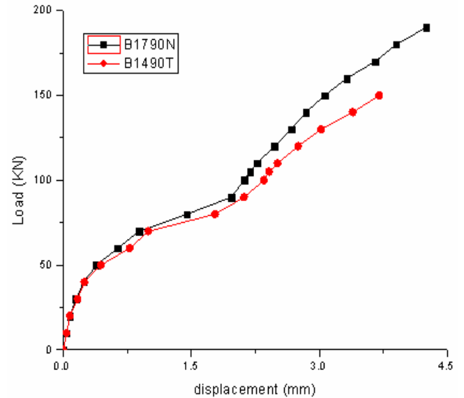
Figure: Result obtained by author to determine the effect of tradition and new effective arrangement on strength of retrofitted beam is shown here
