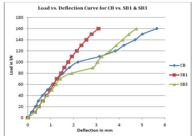
Figure: One of the results obtained by author by comparing control beam and strengthened beam
