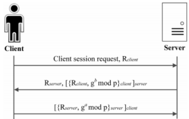
Figure 1: Mutual authentication protocol
