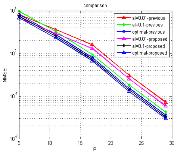
Figure 3: Performance comparison of existing and proposed system for different values of alpha
