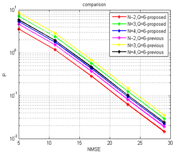
Figure 2: Performance comparison of existing and proposed for different values of Q and N
