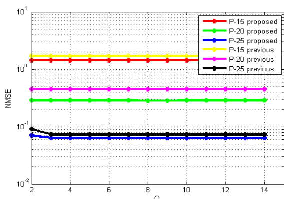
Figure 4 : NMSE versus Q for different P
