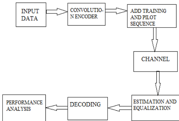
Figure1: Block diagram of the system model
