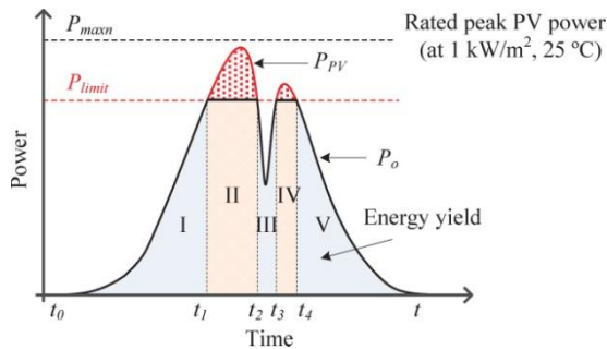
Fig. 2. Operation regions (I, III, V - MPPT; II, IV - CPG) for a single-phase PV system during a day with the proposed control concept, where P_{lim} is determined by the tradeoffs among the device thermal performance, the inverter utilization factor, and the annual energy yield.
