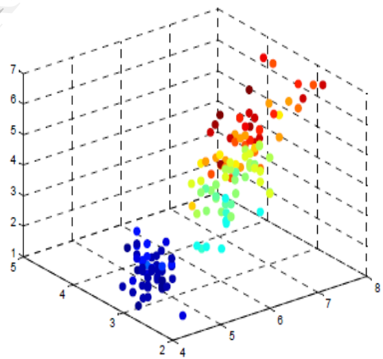
Fig 4: Y-MEAN CLUSTERING WHEN N=25
