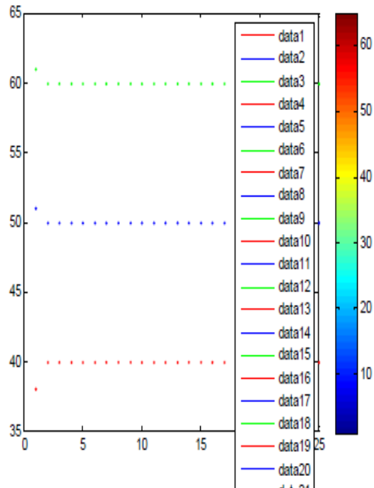
Fig 3: Y-MEAN CLUSTERING
