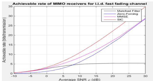
Fig 3: Achievable rate of MIMO receivers for a fast fading channel.
