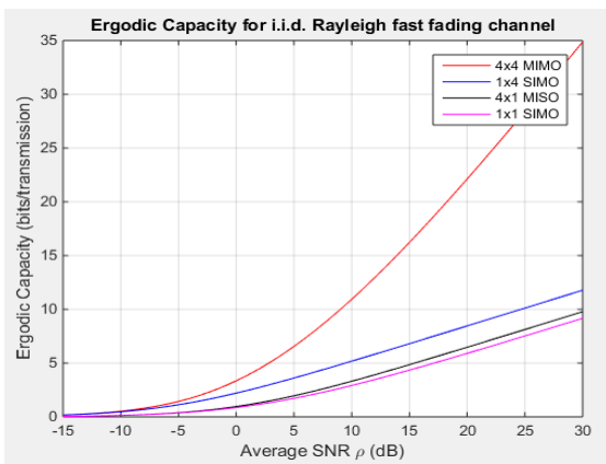
Fig 4: Capacity vs SNR.
