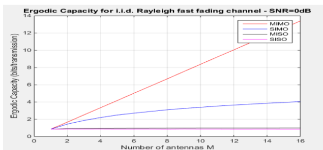
Fig 5: Ergodic capacity vs Number of antennas for different configuration antennas.
