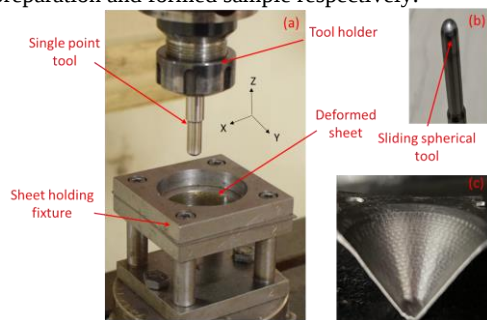
Fig. 2(a) Incremental forming fixture and tooling mounted on the CNC machine; 2(b) single point spherical tool; 2(c) formed sheet
