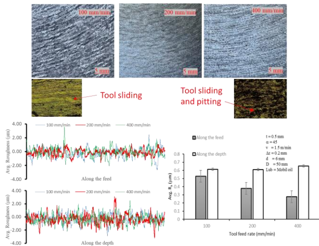
Fig. 6 Surface imagery of the formed sheet with varying tool feed rates; roughness profiles; average roughness values
