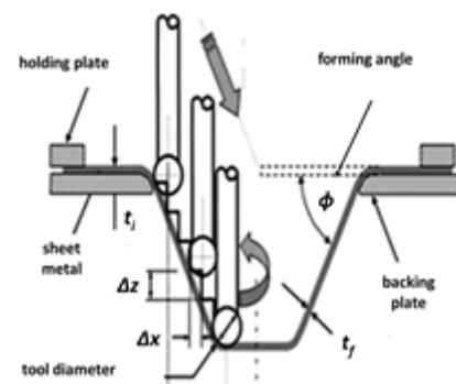
Fig. 1 Schematic of single point incremental forming [2]
