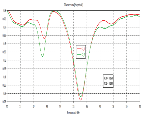
Figure 5 Reflection Coefficient for 1x8 array
