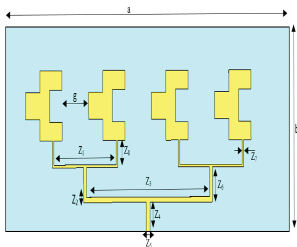
Figure 3 Antenna structure for a 1x4 array
