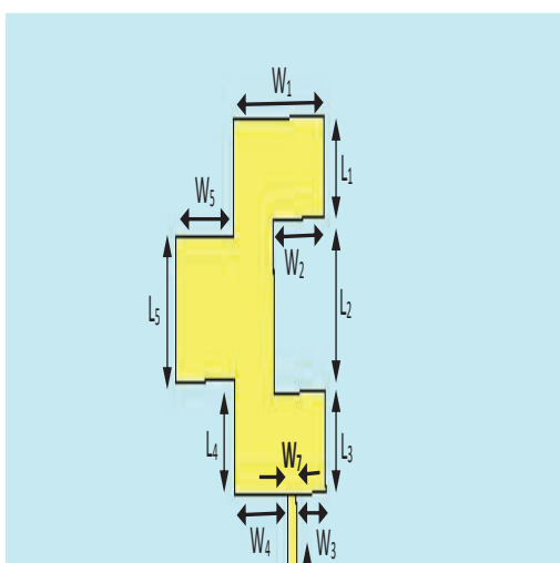
Figure 1 Structure of single patch
