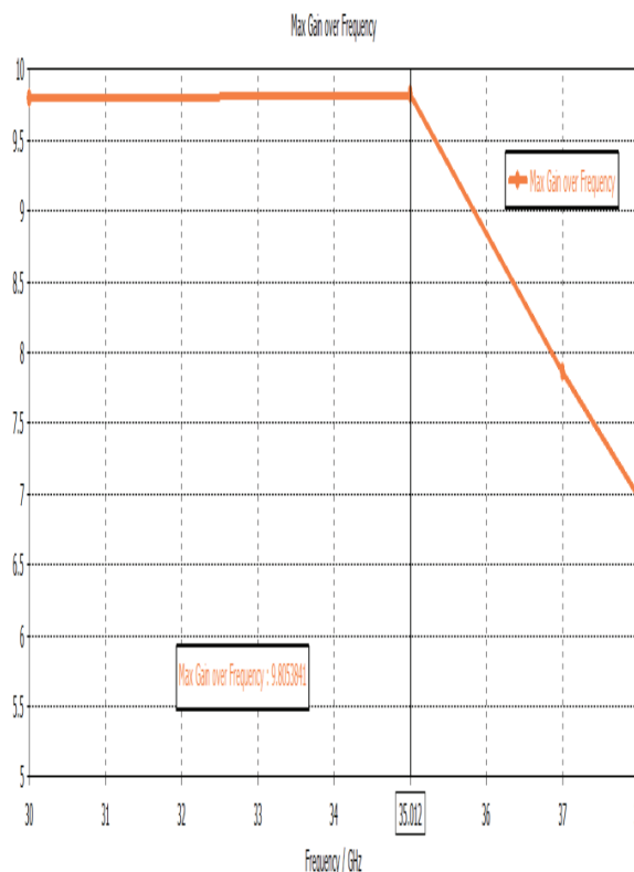
Figure 7 Gain for 1x8 array
