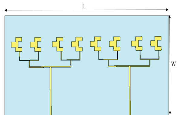
Figure 4 1x8 antenna array
