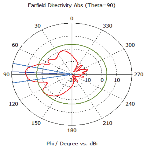
Figure 9 Farfield directivity for Port 1
