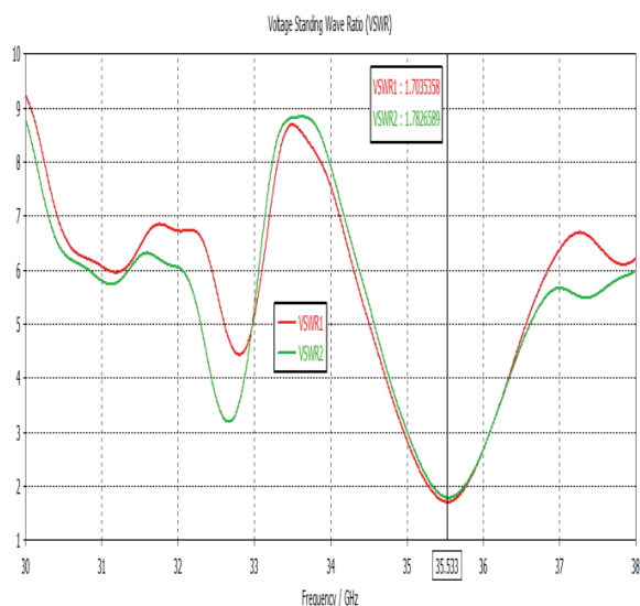
Figure 6 VSWR for 1x8 array
