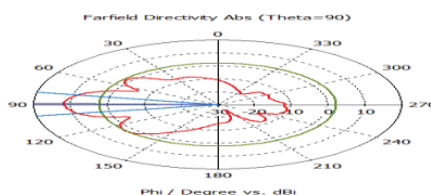
Figure 8 Farfield directivity for Port 1
