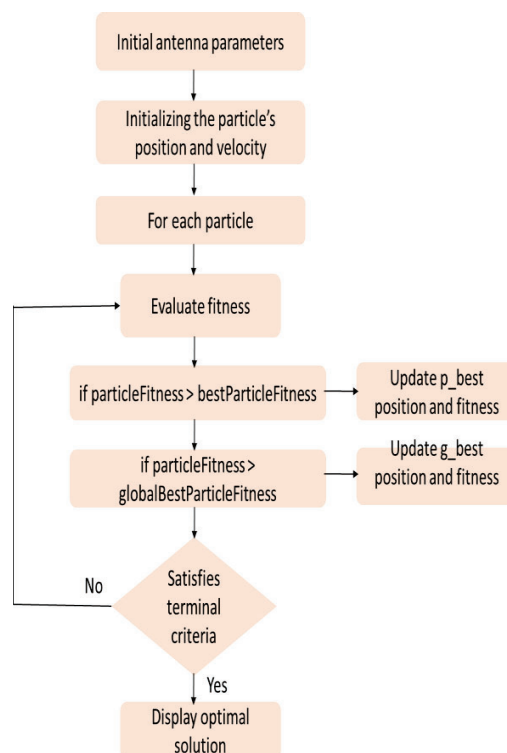
Figure 2 Flowchart of PSO
