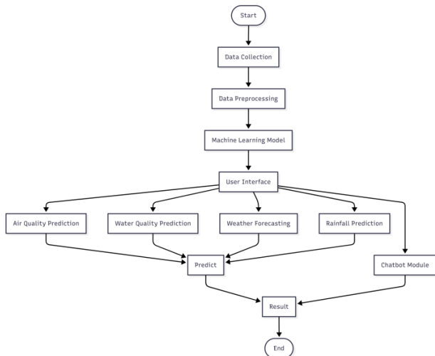
FIGURE1. Software Flowchart
