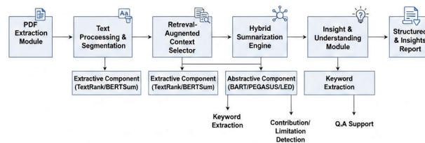
Fig. 1. Proposed Framework for Automated Research Paper Summarization
