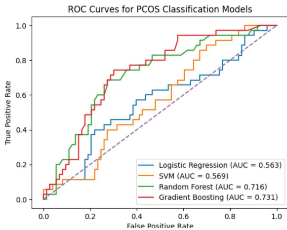
Fig. 4. Receiver Operating Characteristic (ROC) Curves for PCOS classification models. Gradient Boosting achieved the highest discrimination with an AUC of 0.731, followed by Random Forest (0.716), SVM (0.569), and Logistic Regression (0.563).
