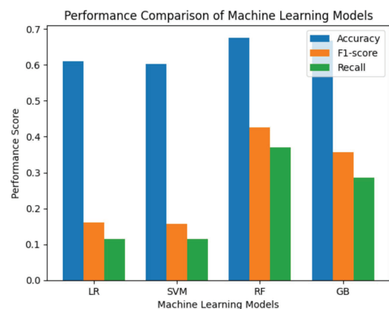
Fig. 3. Performance Comparison of Machine Learning Models (LR, SVM, RF, GB) based on Accuracy, F1-score, and Recall metrics.
