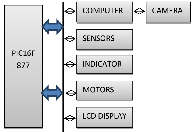
Fig 1. Block diagram of automated gate
